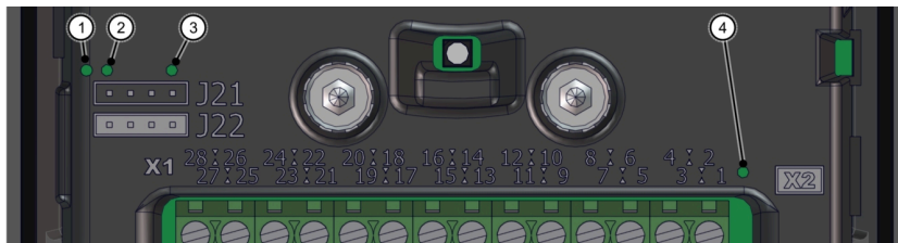
Obr. 12: Stavová LED
