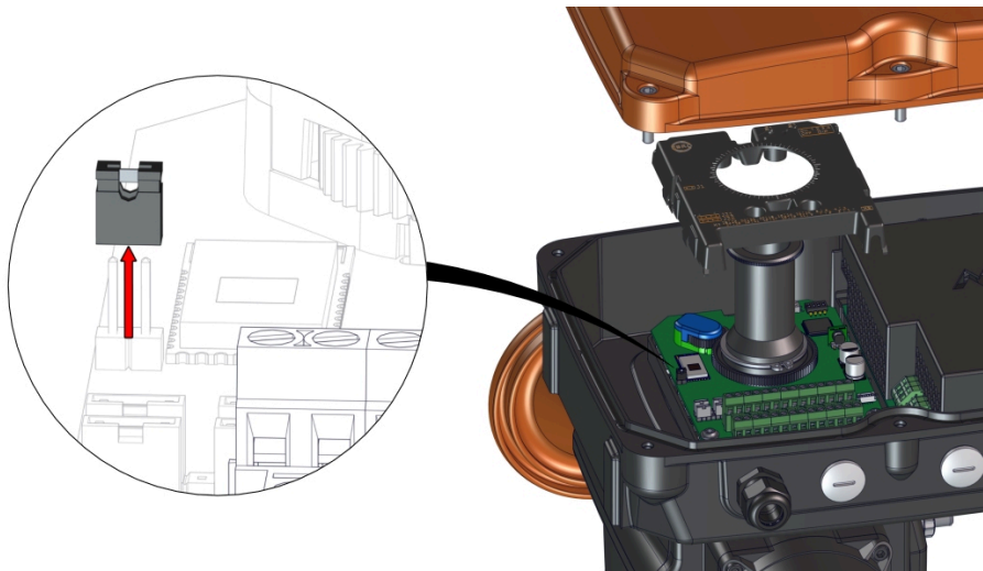
Afb. 15: Jumpers
