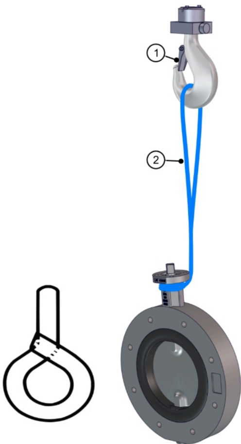
Fig. 6: Lifting full lug-type butterfly valve with a crane
