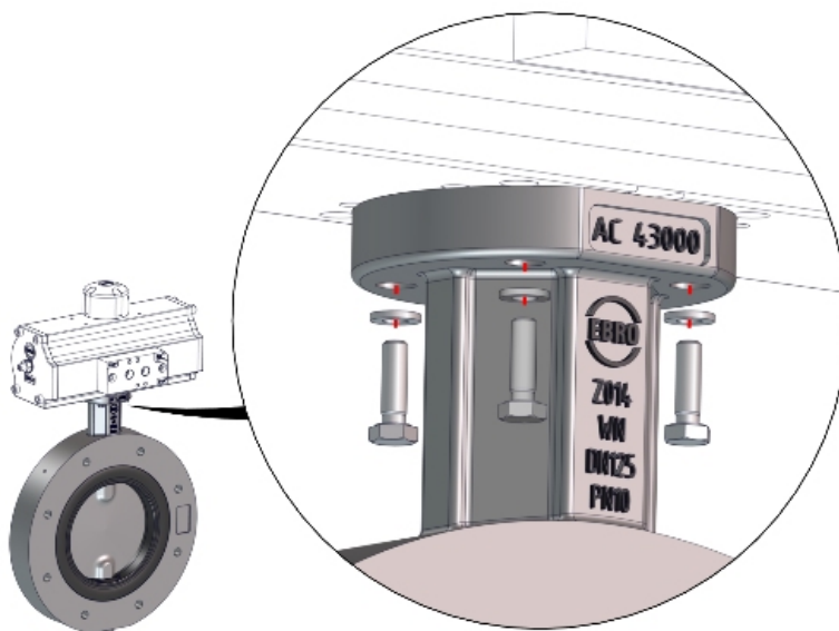
Fig. 7: Principle for mounting components
