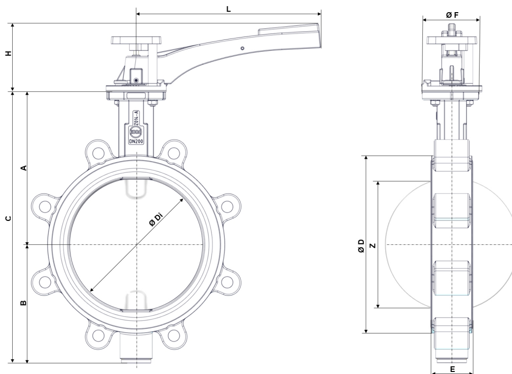
Fig. 3: Main dimensions Z014-A THERM
