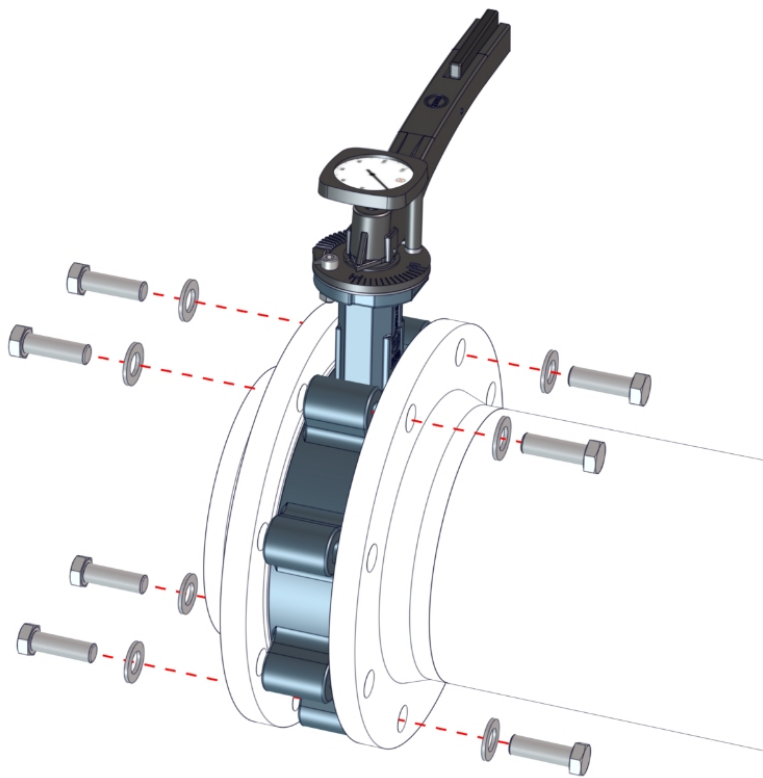
Fig. 8: Positioning the lug-type butterfly valve
