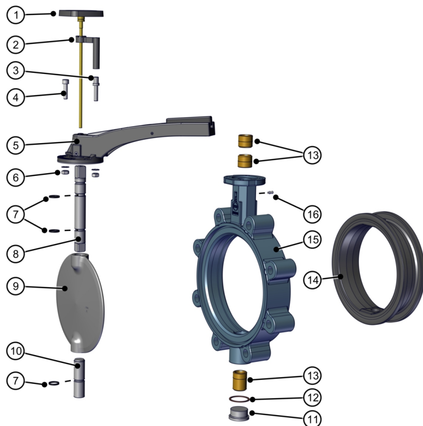
Fig. 16: Bill of materials Z014-A THERM
