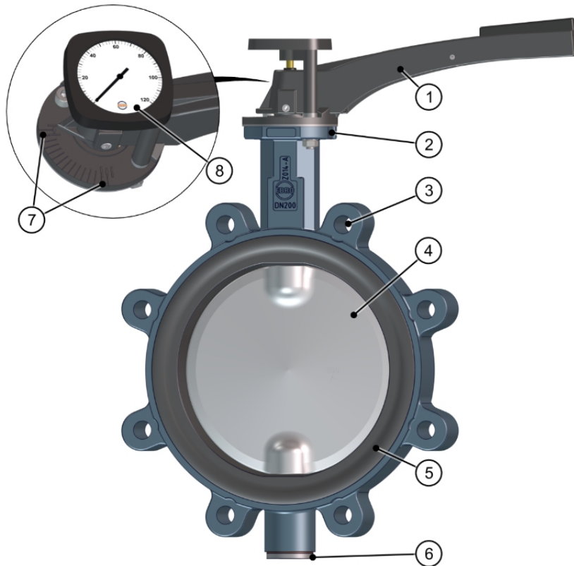
Fig. 2: Components
