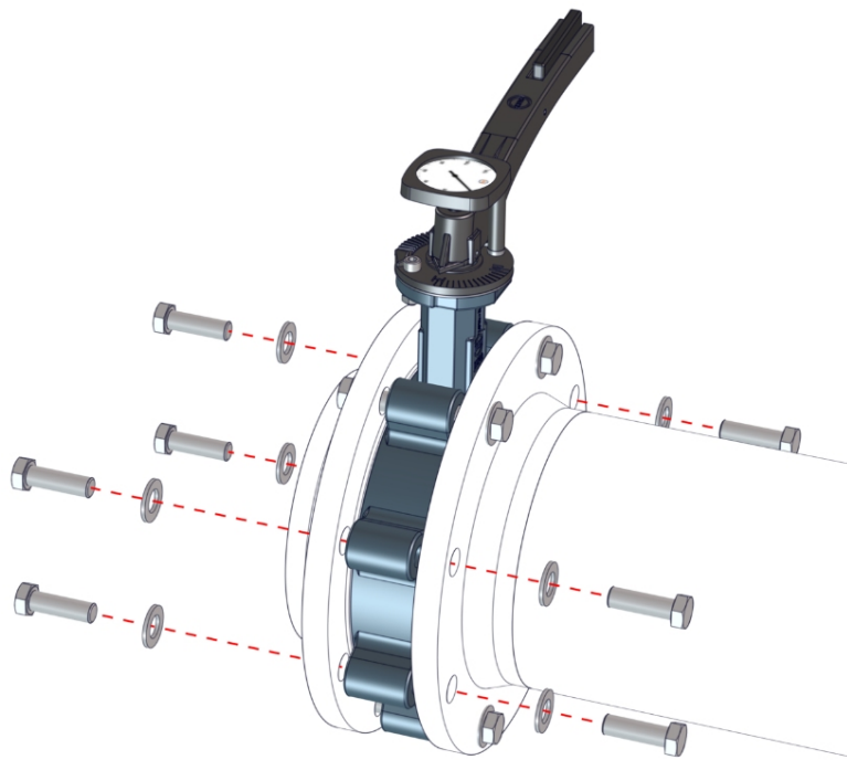
Fig. 9: Screwing on the lug-type butterfly valve
