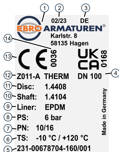
Fig. 1: Example identification plate
