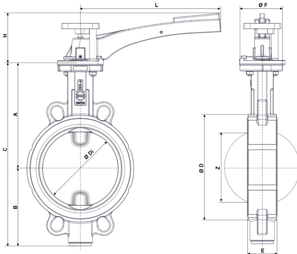
Fig. 3: Main dimensions Z011-A THERM
