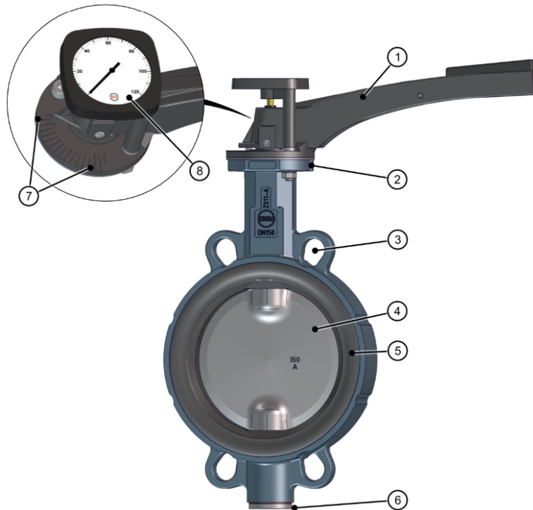
Fig. 2: Components
