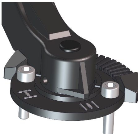
Fig. 15: Position indicator
