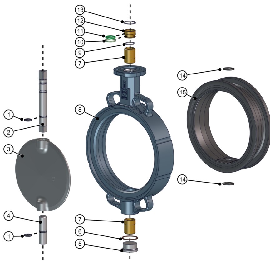
Fig. 17: Bill of materials investment casting disc 2-shaft
