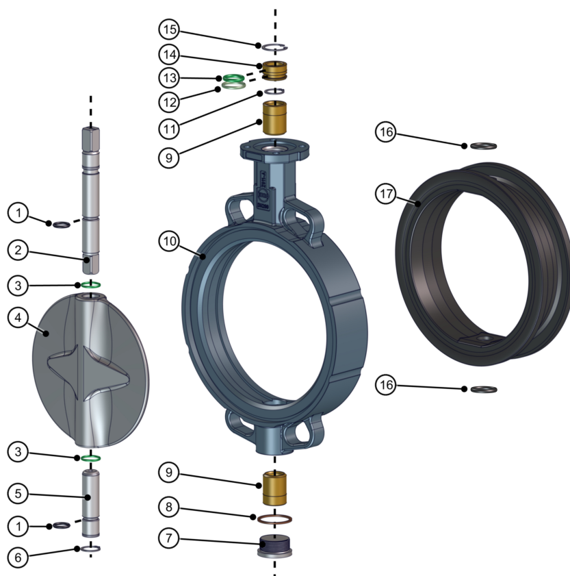
Fig. 19: Bill of materials valve disc 2-shaft
