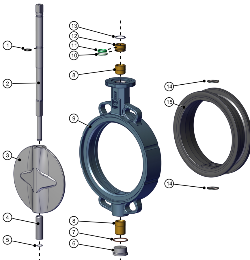
Fig. 18: Bill of materials valve disc 1-shaft
