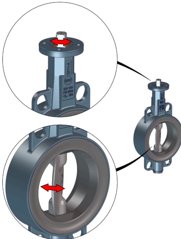
Fig. 4: Moving parts
