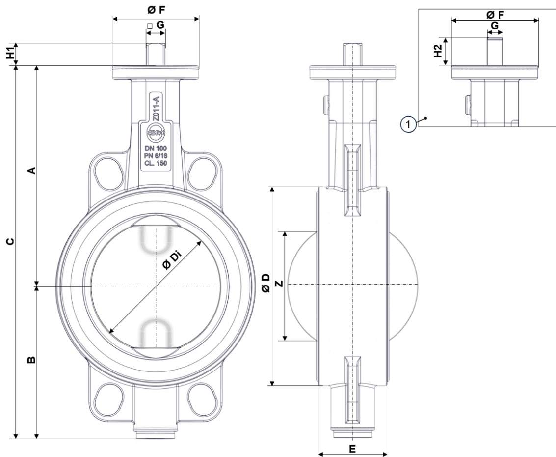
Fig. 3: Main dimensions Z011-AS
