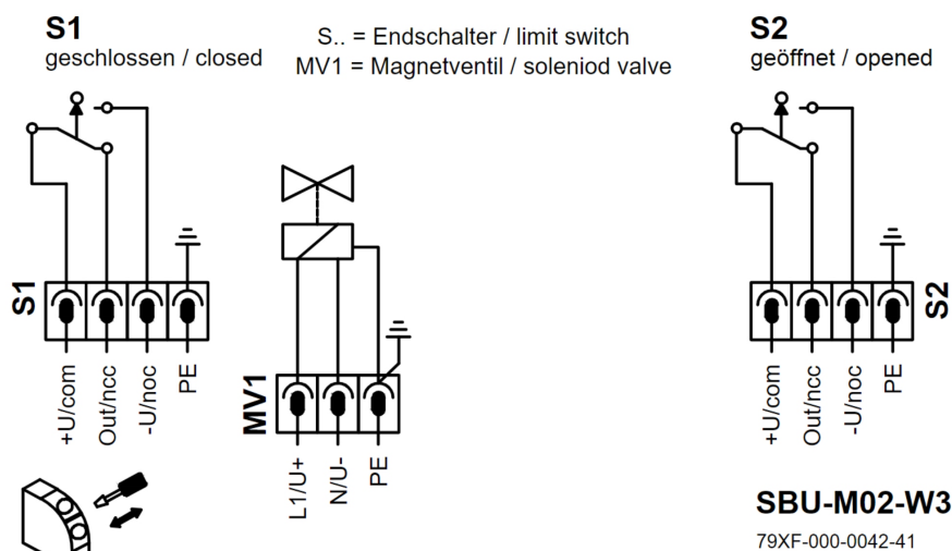
Fig. 7: Circuit diagram SBU Basic
