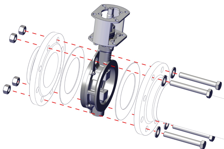
Figur 8: Placer mellemflangeklap
