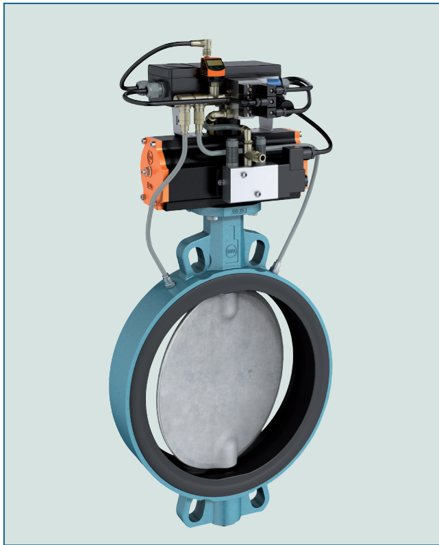
Resilient seated butterfly valve type Z011-A with inflatable liner.
