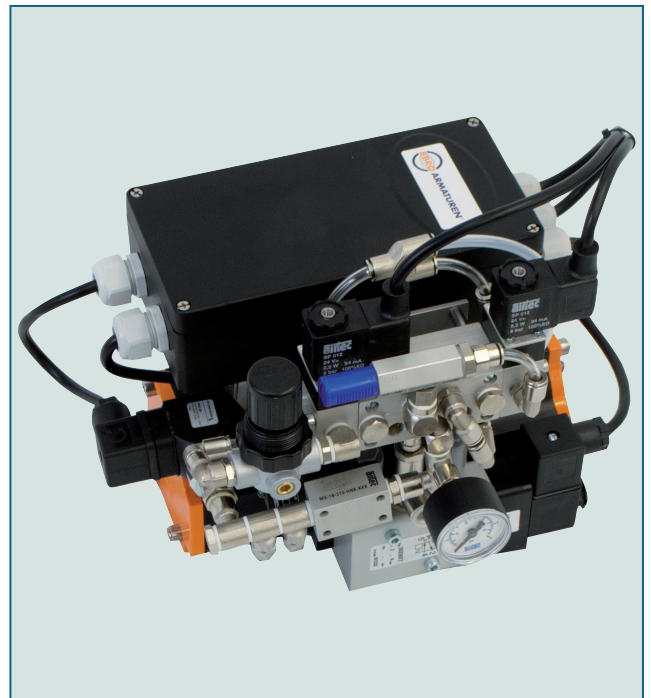
EBRO pressure control/-monitoring
